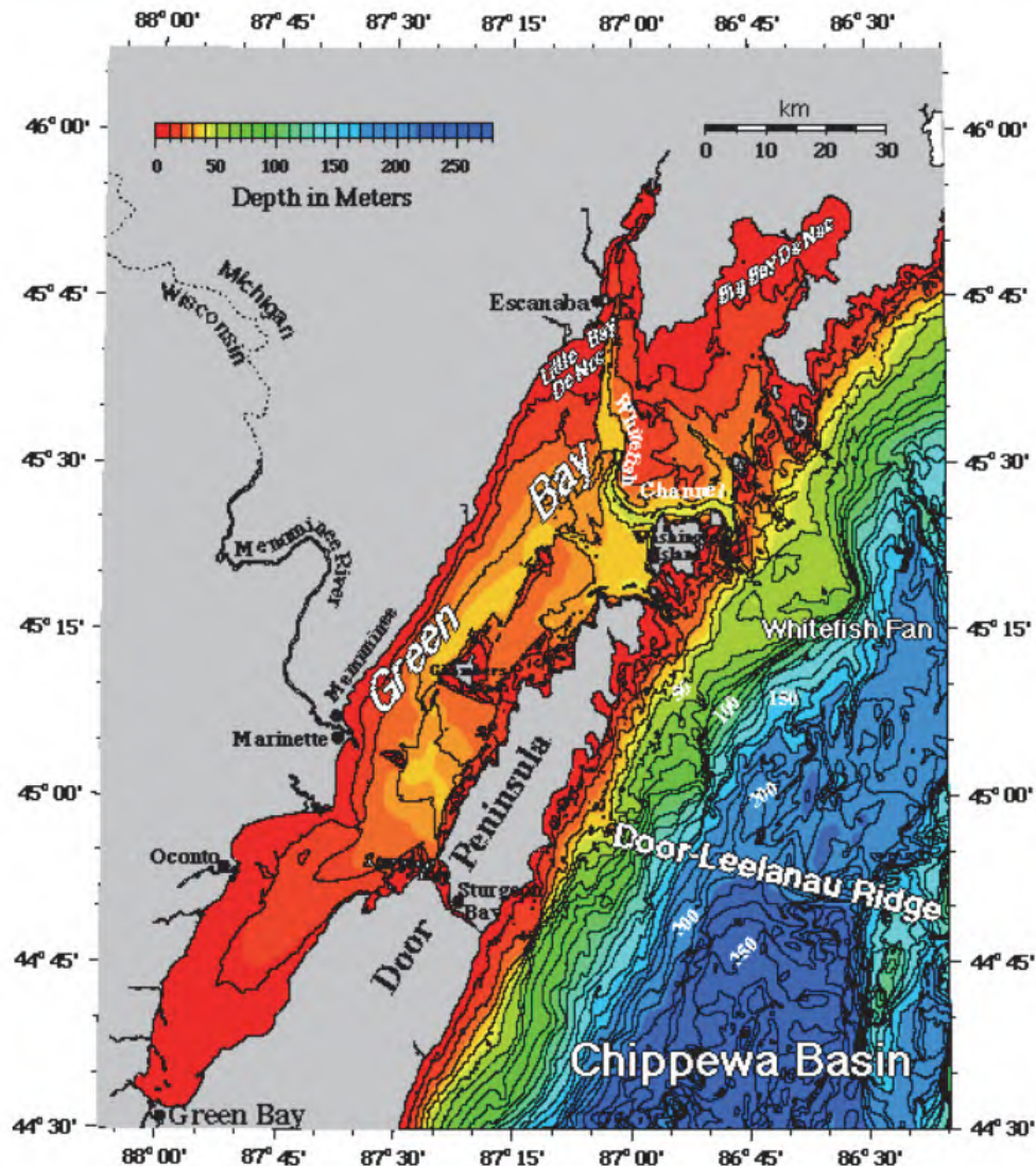
Figure 23. Bathymetric contours for Green Bay, Lake Michigan (from: http://www.ngdc.noaa.gov/mgg/greatlakes/lakemich_cdrom/html/area1.htm ).
