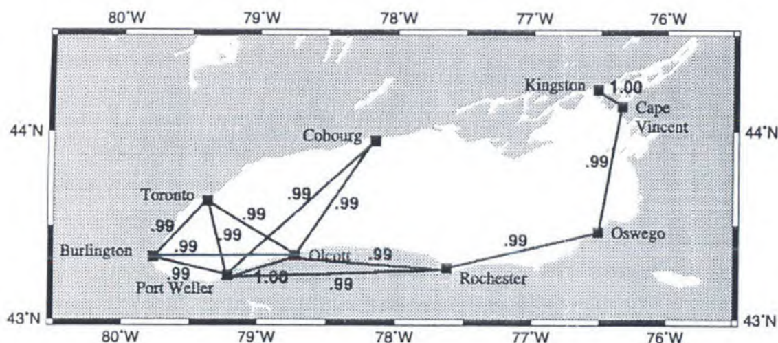
Figure 45. Lake Ontario correlation coefficients from Zervas (1997).
