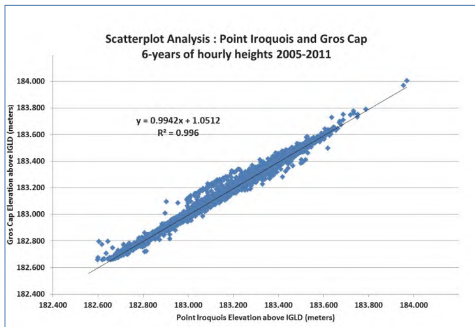
Figure 11. X-Y plot scatterplot comparison of hourly heights for Gros Cap and Point Iroquois.
