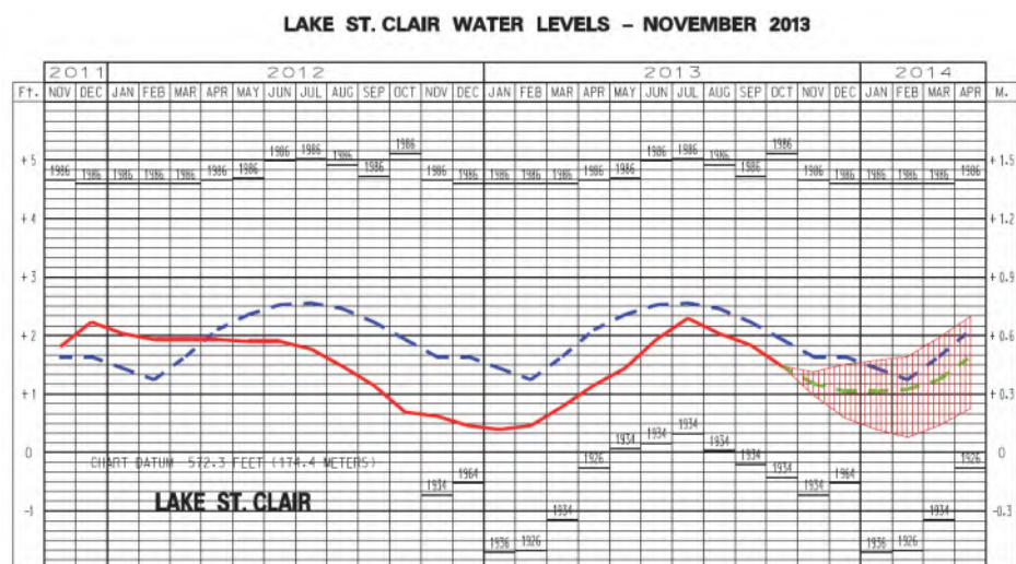
Figure 6c. USACE water level bulletin for Lake St Clair for November 2013.
