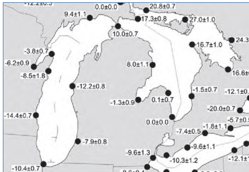
Figure 25. Relative vertical velocities (in cm/century) for Lake Michigan and Lake Huron (Mainville and Craymer [2005]) relative to the lake outlet.
