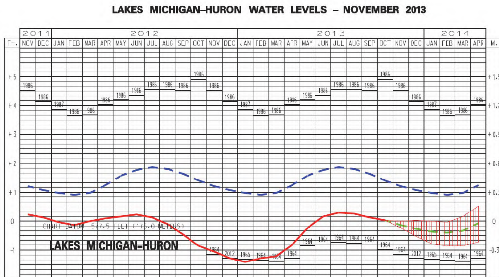
Figure 6b. USACE water level bulletin for Lakes Michigan-Huron for November 2013.
