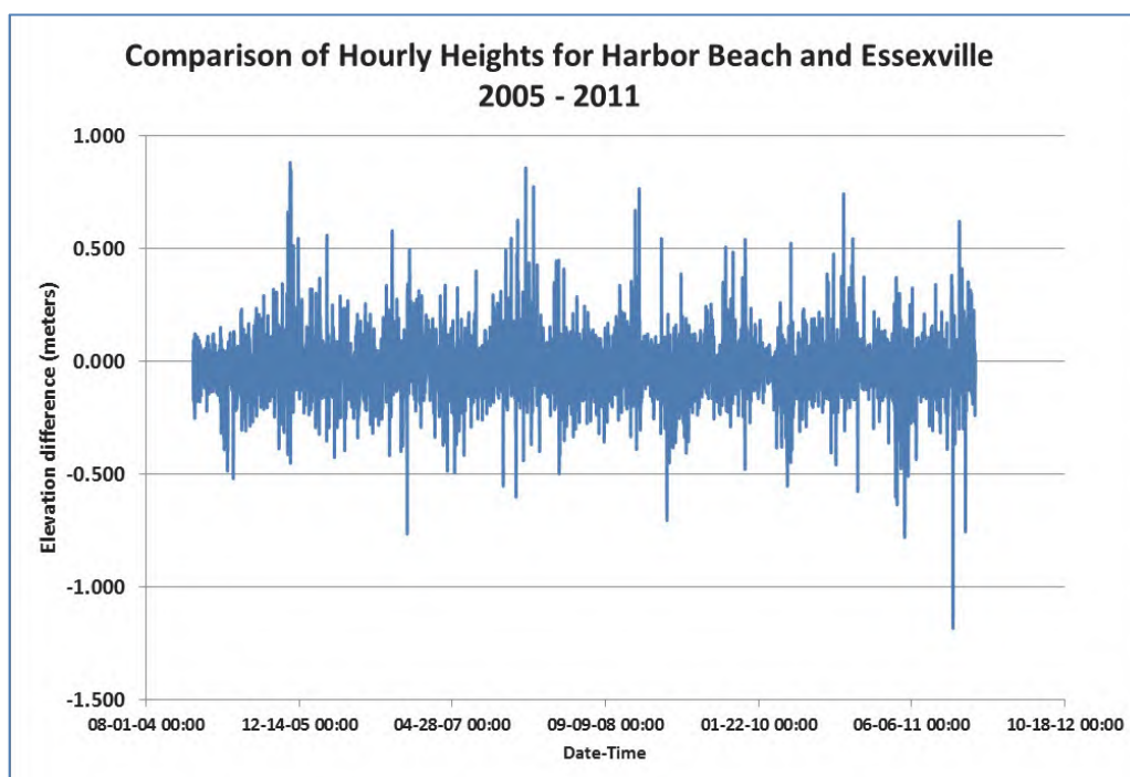
Figure 12. Hourly height differences between Harbor Beach and Essexville, 2005-2011.
