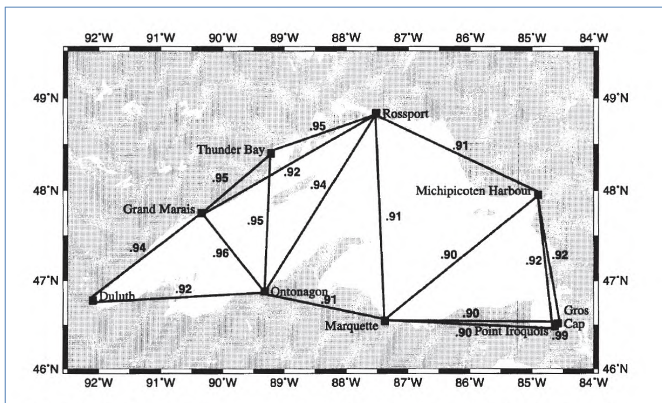
Figure 16. Lake Superior correlation coefficients from Zervas (1997).
