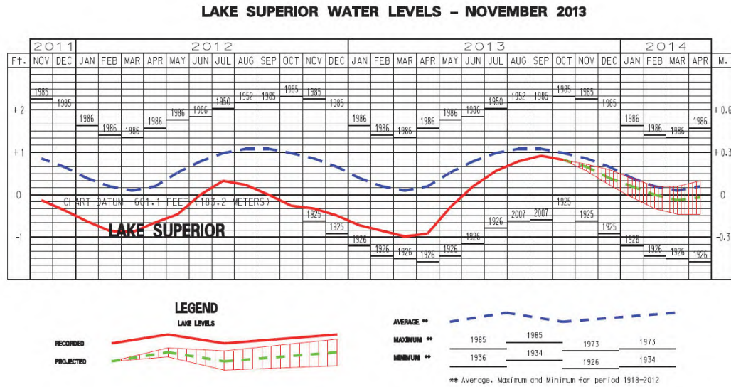
Figure 6a. USACE water level bulletin for Lake Superior for November 2013. Legend depicted is common to all following bulletin plots.
