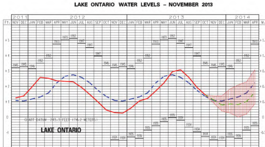
Figure 6e. USACE water level bulletin for Lake Ontario for November 2013.
