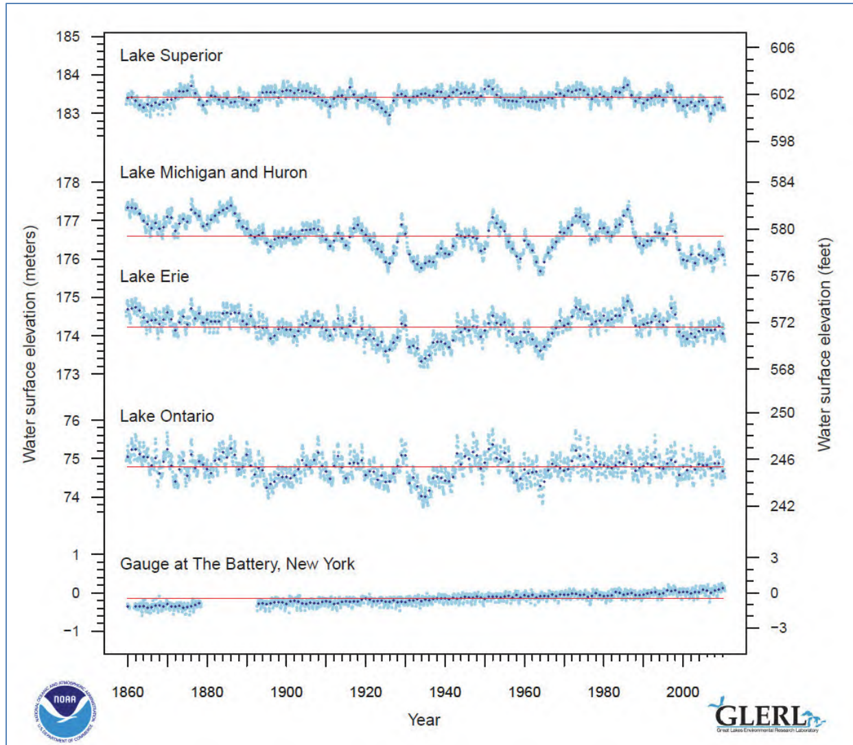
Figure 5. Comparison of long-term hydrographs of each Great Lake with long-term sea level variations at New York City (from GLERL, 2013).
