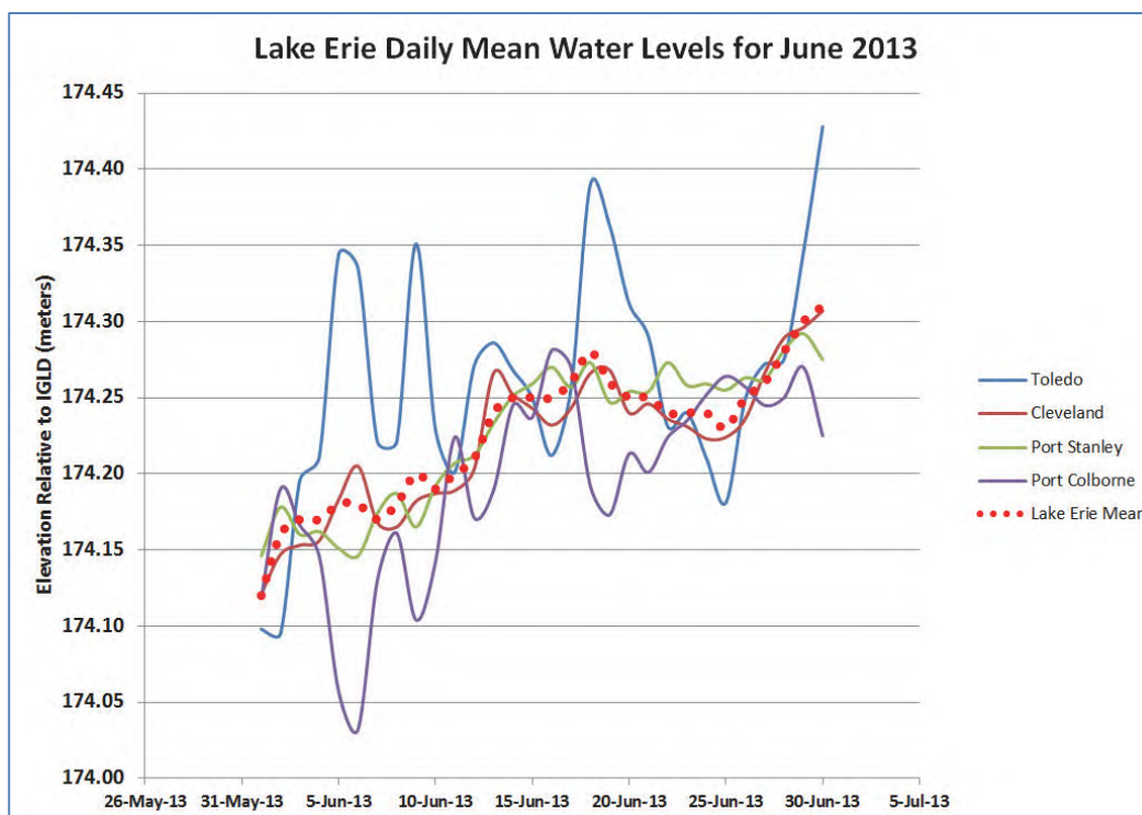
Figure 38. Lake Erie daily mean water Levels June 2013.
