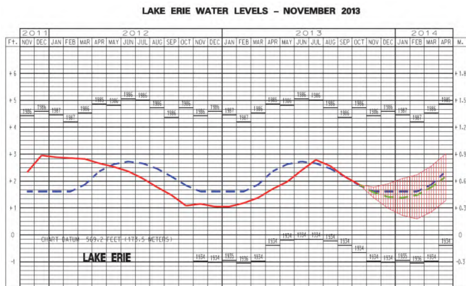
Figure 6d. USACE water level bulletin for Lake Erie for November 2013.
